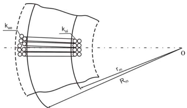
Fig. 1 Constructive features of the toroidal winding
