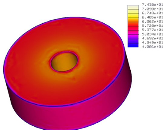
Fig. 3 Temperature distribution on the toroidal transformer
