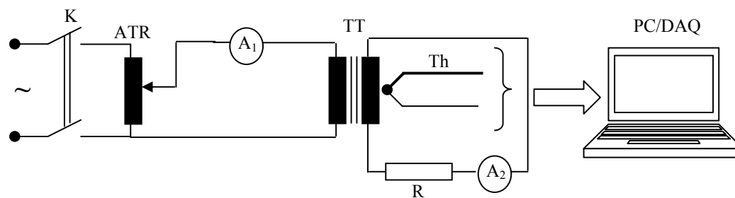
Fig. 12 Main electric diagram for experimental tests
