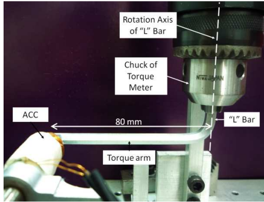
Fig. 8 Torque arm of the "L" bar
