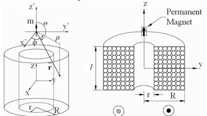
Fig. 5 Air-core coil [6]
