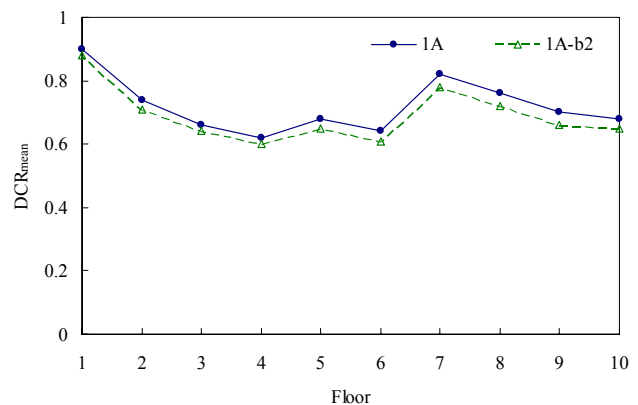
Fig. 4(c) Mean DCRs for Case 1A
