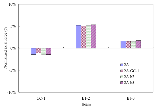
Fig. 5(b) Axial force of beams connected with the Case 2A column-removed point
