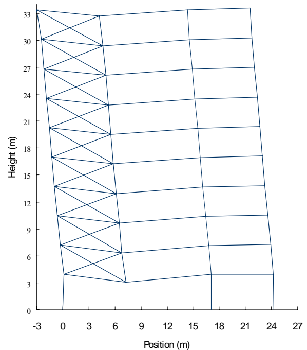
Fig. 8 Flexural deformation of the column lines
