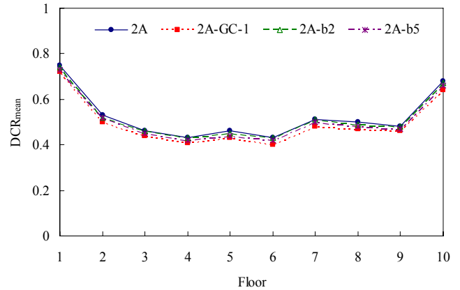
Fig. 4(b) Mean DCRs for Case 2A
