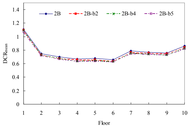
Fig. 4(e) Mean DCRs for Case 2B (continued)
