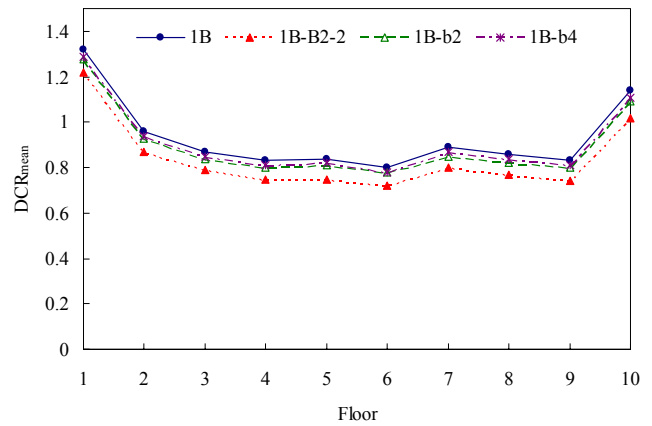
Fig. 4(a) Mean DCRs for Case 1B
