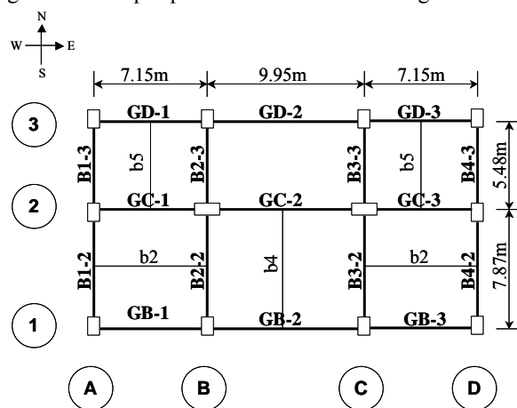
Fig. 1 Plan dimensions of the building
