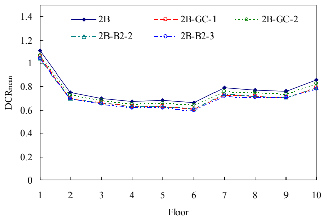
Fig. 4(d) Mean DCRs for Case 2B
