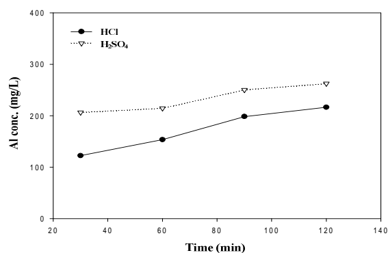
Fig. 2 Relationship between dissolved aluminum concentration and reaction time
