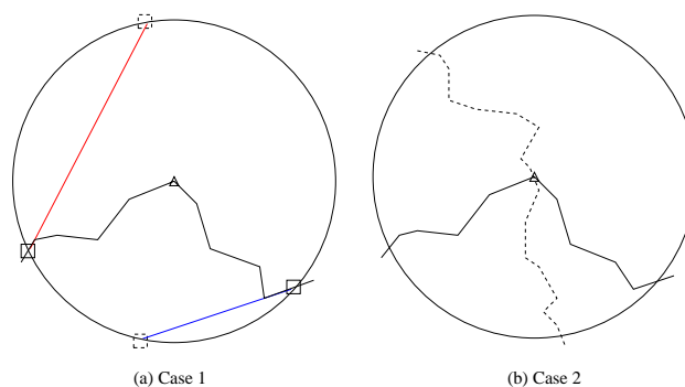
Fig. 2. The relationship between the line segments and the circle. The center of the circle is marked by a triangle symbol.
