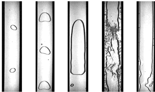
Fig. 1 The classification of the flow patterns observed in the experiment B - bubble, C - cup-bubble, P - slug, F - slug-churn, A - annular
