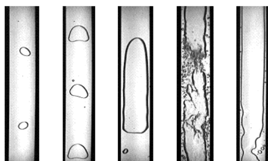
Fig. 1 The classification of the flow patterns observed in the experiment
