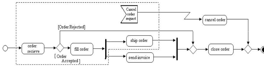
Fig. 4 A sample Activity diagram [3]
