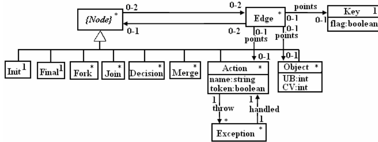
Fig. 2 Proposed type graph for UML 2.0 Activity diagram
