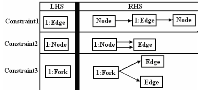
Fig. 3 Three atomic graph constraints
