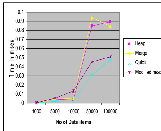
Fig. 1 Sorting Algorithms Performance Category-I
