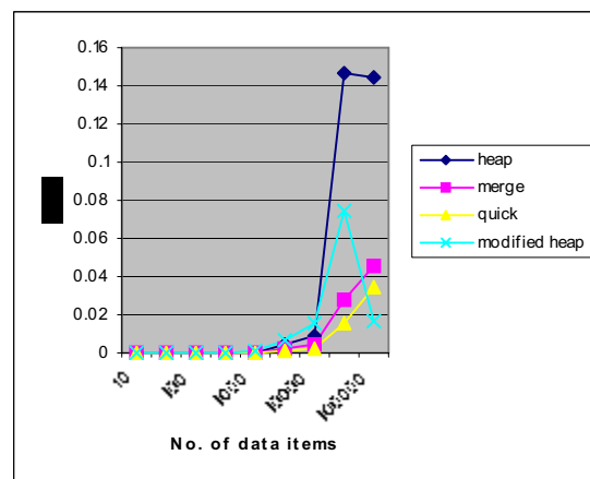
Fig. 2 Sorting Algorithms Performance Category-II
