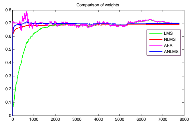
Fig. 7 Comparative analysis of evaluation of filters taps
