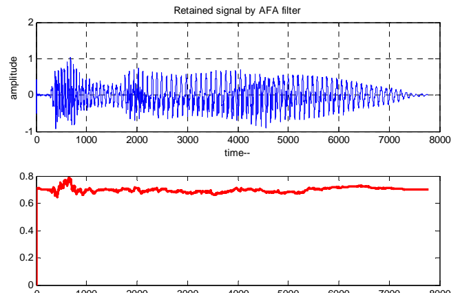
Fig. 5 Filtered output and time evolution of filter taps for AFA algorithm
