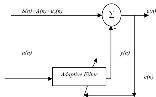
Fig. 1 An adaptive noise cancelling system
