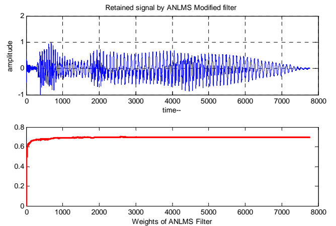
Fig. 6 Filtered output and time evolution of filter taps for ANLMS algorithm
