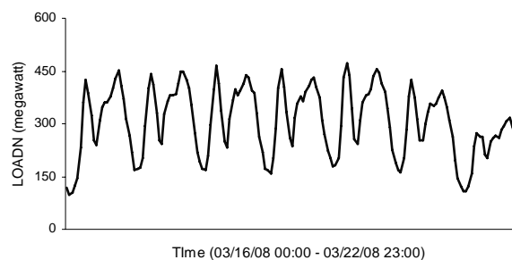
Fig. 1 Weekly hourly load curve of the Italian railways - North Zone of the GME
