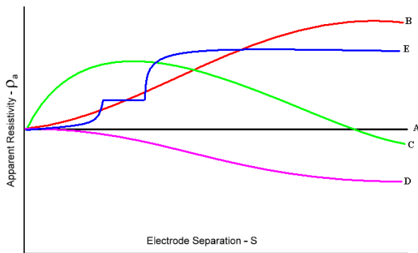
Fig. 1 IEEE 80 soil structure
