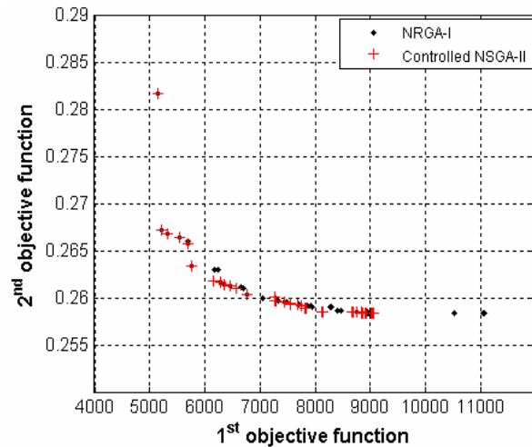
Fig.4 An example for non-dominated solutions problem
