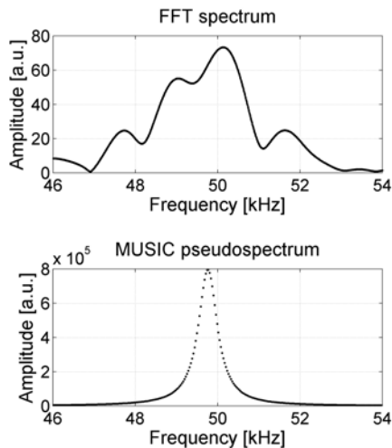
Fig. 5. Corresponding spectra to figure 4, calculated using FFT and MUSIC. The results are f = 50.13 kHz for the FFT (predicted: f = 50.11 kHz) and f = 49.77 kHz for the MUSIC algorithm (predicted: f = 49.94 kHz).
