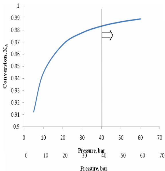
Fig. 2 Simulated effect of pressure on Conversion at 360^\circ\text{C}
