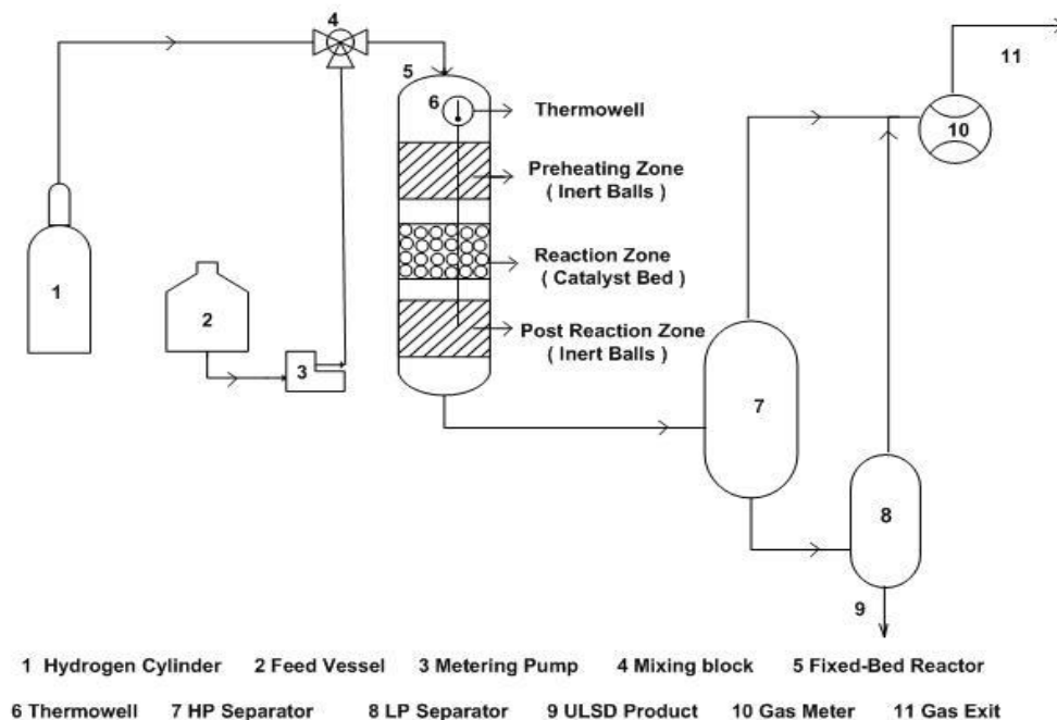
Fig. 1 Experimental setup
