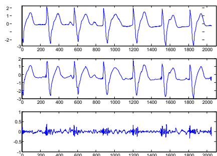
Fig. 3 – Compressing ECG using the cardbal2 with Id prefiltering method. The above figure shows the original signal, the middle shows reconstructed signal after compression and the bottom shows error between them. The first 2048 samples of MIT-BIH record 107 are used. CR=16.384, PRD=7.8842%, CC=99.6612%, D=0.006216.
