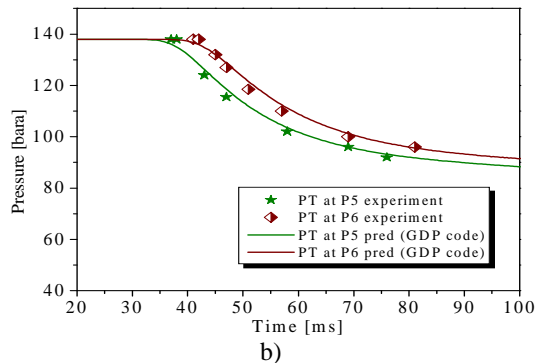
Fig. 4 Pressure time history at PT-P1&P8 (a) and PT-P5&P6 (b) case 2
