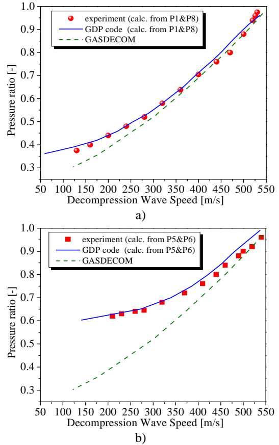
Fig. 7 Decompression wave speed as a function of pressure ratio
