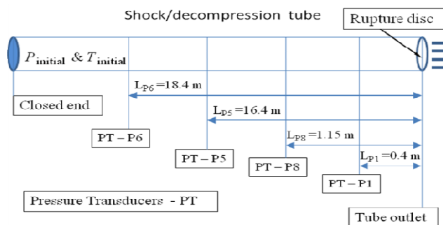
Fig. 1 Schematic of the experimental decompression tube
