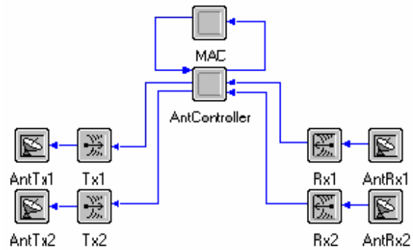
Fig. 3 a) BS node model
