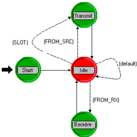
Fig.4 b) Wireless Terminal MAC process model
