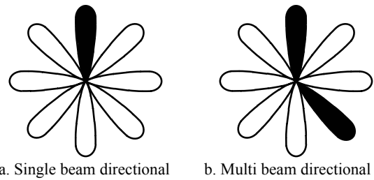
Fig. 2 Switched beam directional antenna
