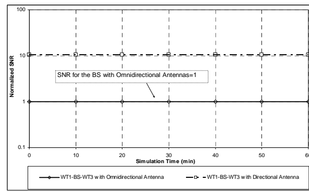
Fig. 8 Normalized SNR results for the wireless network utilising directional antenna
