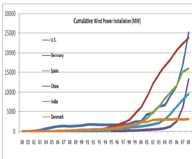
Fig. 3 Cumulative Wind Power Capacity [7][18][19][20][21][22][23]
