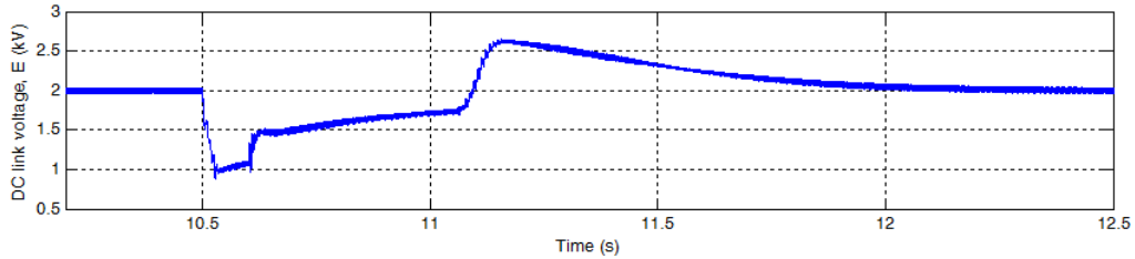
(d) DC link voltage response to three-phase fault at 10.5 s
