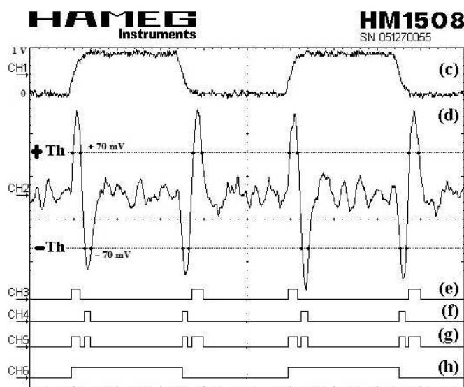
Fig. 6 Detection process
