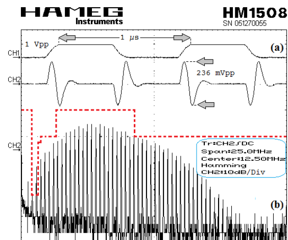
Fig. 4 (a) Experimental signals V_{in} and V_{out} (b) PSD of the pulse sequence
