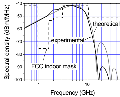
Fig. 3 PSD of the pulse
