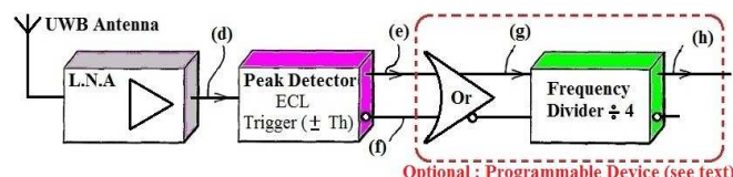
Fig. 5 UWB receiver based on ECL for monocycle pulses (LNA: Low Noise Amplifier)
