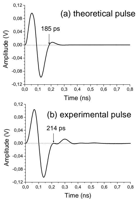
Fig. 2 The generated pulse
