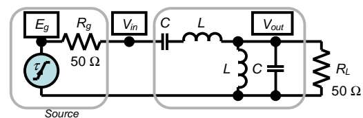
Fig. 1 The monocycle pulse generator
