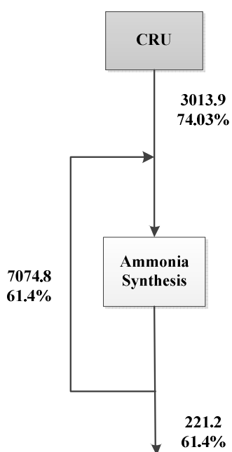
Fig. 5 Hydrogen network of ammonia complex
