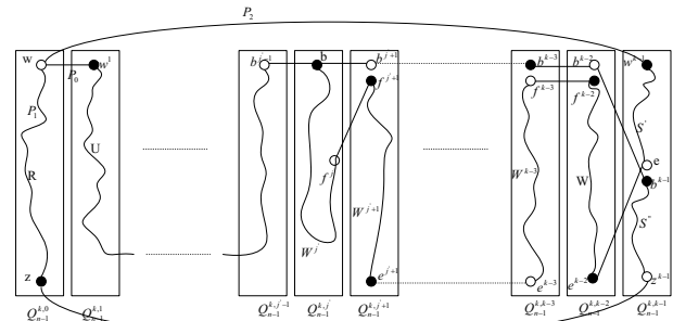
Fig. 13. The illustration for Case 4.1 of Theorem 3.
