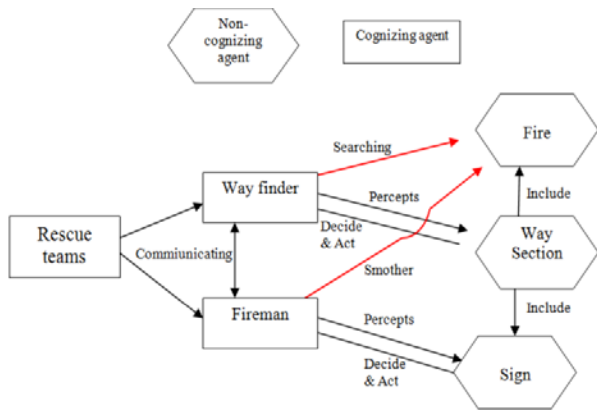
Fig. 4 Conceptual model of multi-agent rescue operation
