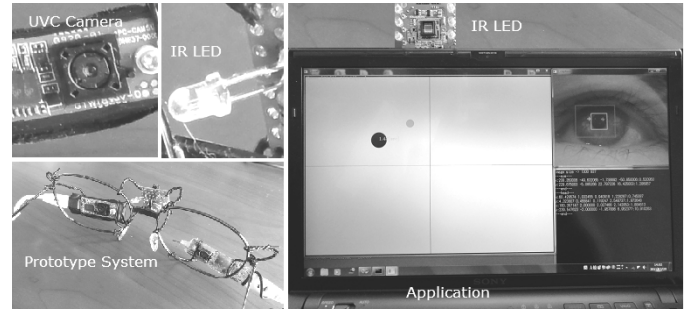
Fig. 4. Experimental system
