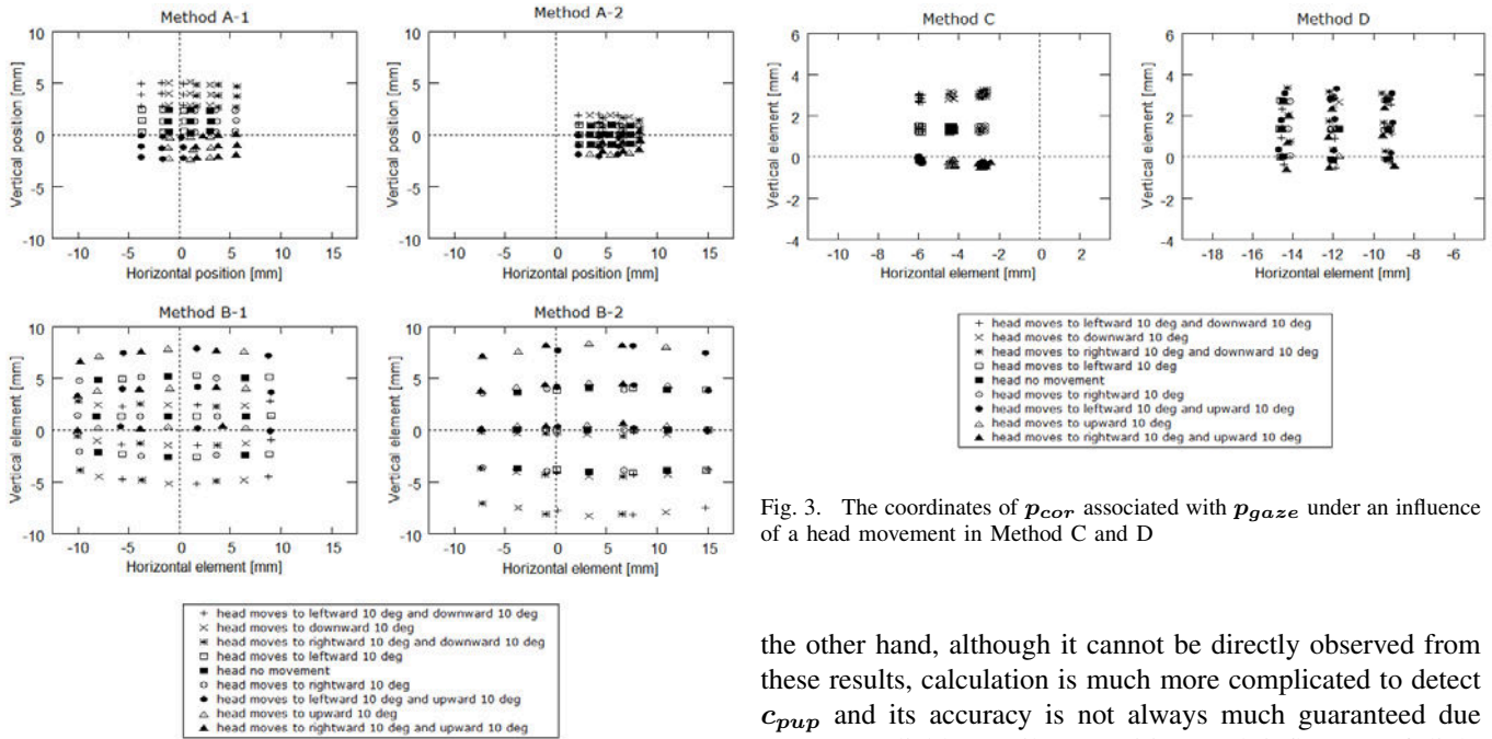
Fig. 2. The coordinates of p_{cor} associated with p_{gaze} under an influence of a head movement in Method A and B
