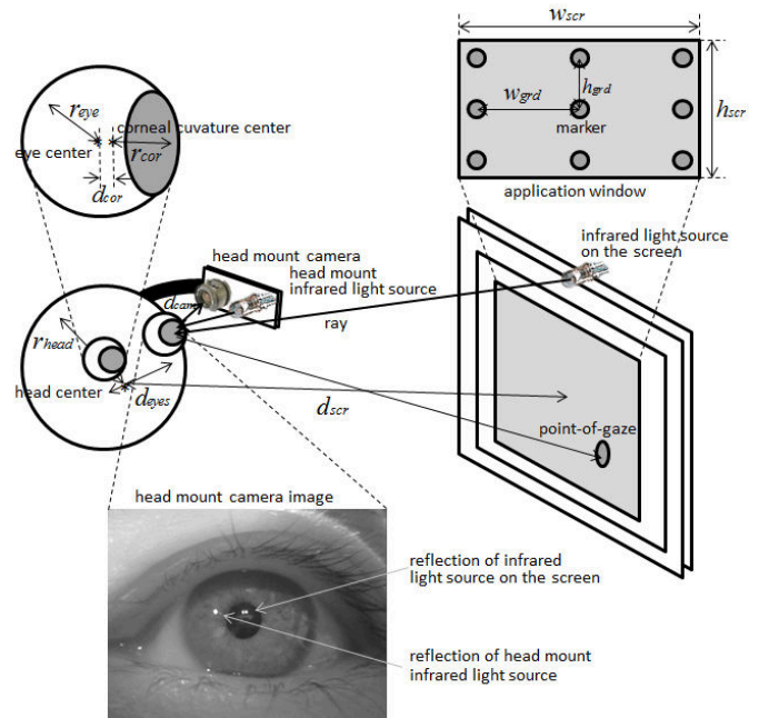
Fig. 1. Eye tracking system diagram
