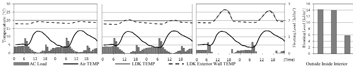
(1) Outside Insulation (2) Inside Insulation (3) Interior Insulation (4) AC Load of 9-10.Jan. Fig. 4 Relation Between Walls-Surface Temperature and Heating Load (Middle Unit, South-Facing, AC④, 9-10.Jan.)
