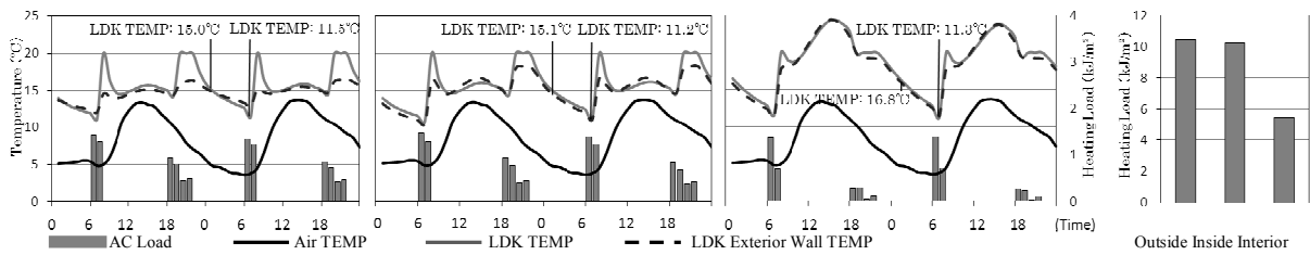
(1) Outside Insulation (2) Inside Insulation (3) Interior Insulation (4) AC Load of 9-10.Jan. Fig. 3 Relation Between Walls-Surface Temperature and Heating Load (Middle Unit, South-Facing, AC①, 9-10.Jan.)
