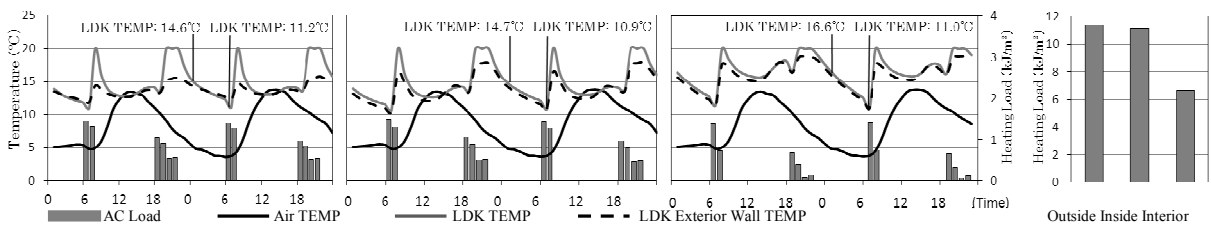
(1) Outside Insulation (2) Inside Insulation (3) Interior Insulation (4) AC Load of 9-10.Jan. Fig. 5 Relation Between Walls-Surface Temperature and Heating Load (Middle Unit, West-Facing, AC①, 9-10.Jan.)
