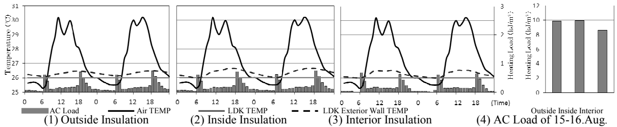
Fig.8 Relation Between Walls-Surface Temperature and Heating Load (Middle Unit, South-Facing, AC④, 15-16.Aug.)
