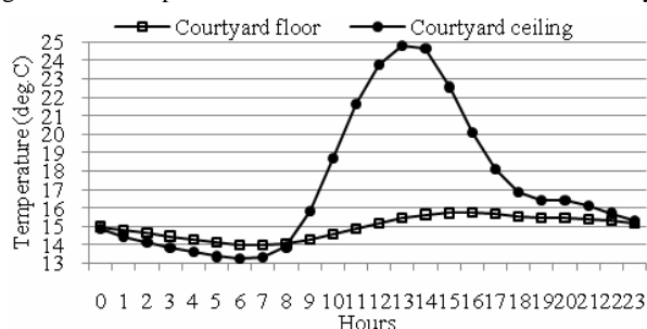
Fig. 12 Mean temperatures of Wellington 'wind-rain' house' courtyard
