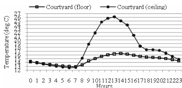
Fig. 11 Mean temperatures of Auckland 'wind-rain' house' courtyard
