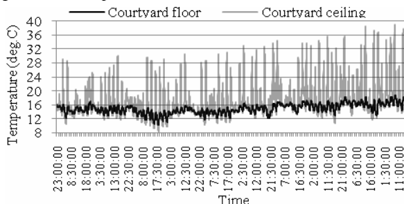
Fig. 10 Indoor temperatures of Wellington 'wind-rain' house's courtyard
