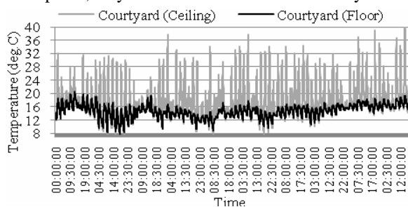
Fig. 9 Indoor temperatures of Auckland 'wind-rain' house' courtyard
