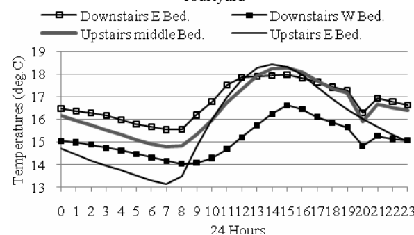
Fig. 13 Mean temperatures of upstairs and downstairs bedrooms
