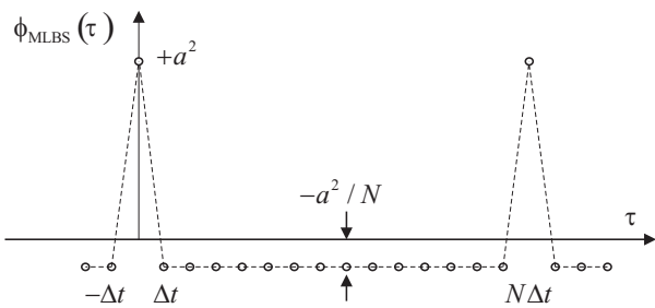
Fig. 2. Shape of auto-correlation function of MLBS.
