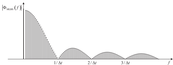
Fig. 3. Shape of power spectrum of MLBS.
