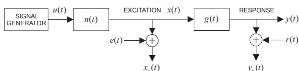
Fig. 1. Typical FRF-measurement arrangement.
