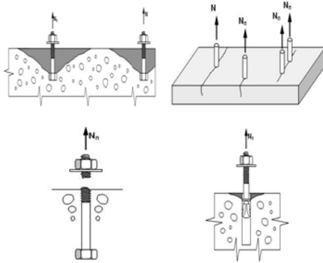
Fig. 2 Tensile Failure Mechanism for Post-Installed Anchor Systems
