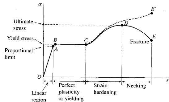
Fig. 8 Steel Material Nonlinear Model
