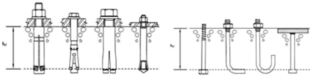
Fig. 1 Variety of Post-Installed Anchor
