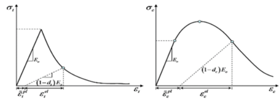
Fig. 7 Concrete Material Nonlinear Model
