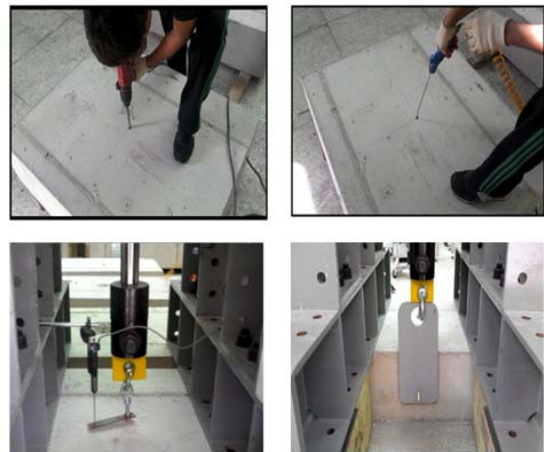
Fig. 4 Test Setup for Post-Installed Anchor Systems
