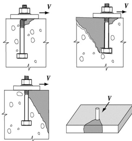
Fig. 3 Shear Failure Mechanism for Post-Installed Anchor Systems
