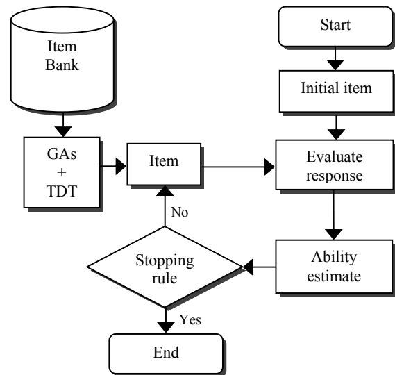
Fig. 1 CAT Flowchart.
