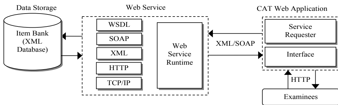
Fig. 2 System Architecture.
