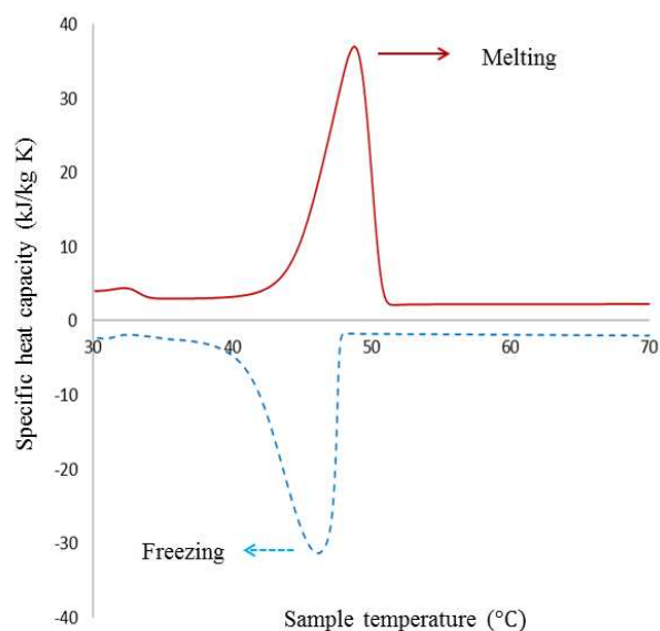
Fig. 2 DSC results for paraffin wax
