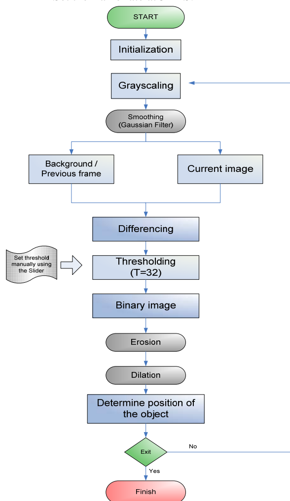
Fig. 9 Program flow chart
