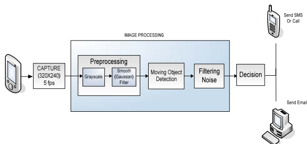
Fig. 2 Overall system architecture block diagram
