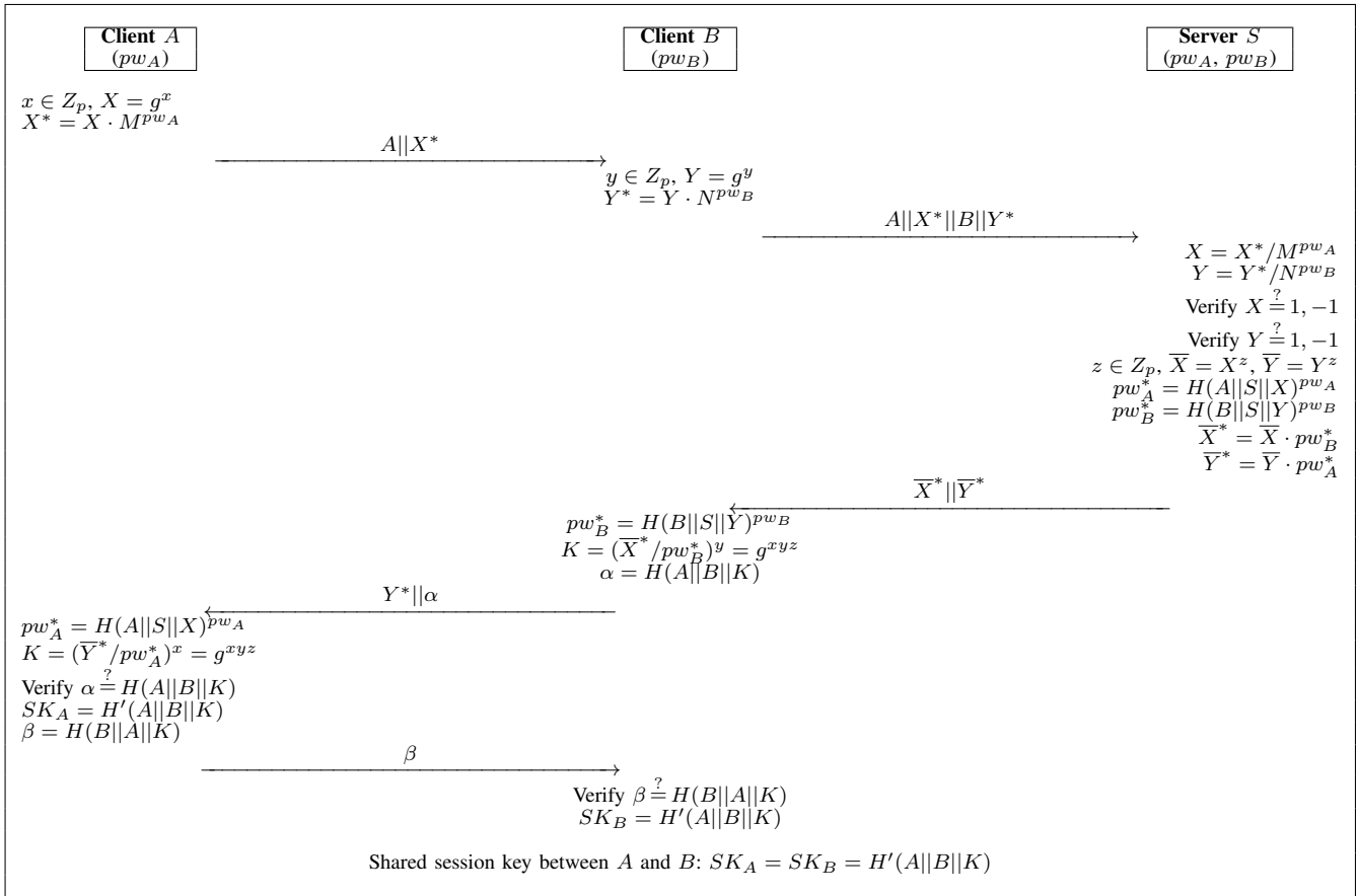
Fig. 1. Debiao-S-3PAKE protocol
