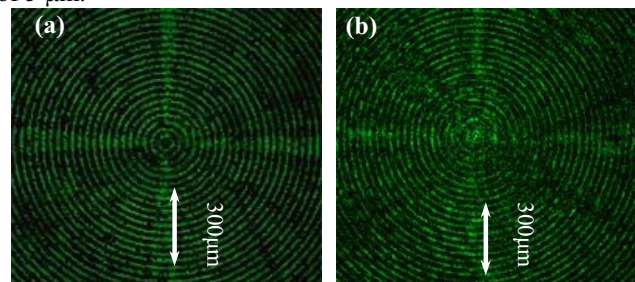
Fig.3 (color online). Self replication of circular mask at different Talbot distances: (a) Z_T = 0 and (b) 20Z_T = 31.40 \pm 0,01 \text{ mm} .
