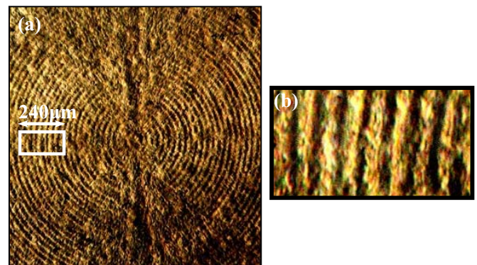
Fig.7 (Color online) Phase microscope image of photonic lattices recorded inside the LN:Fe crystal by annular mask: (a) replicated image at the exit surface of the crystal. (b) Enlarged image of the region marked by white rectangle in (a)
