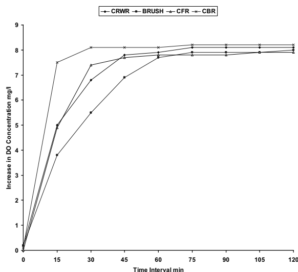
Fig. 7 Variation of Dissolve Oxygen with Time for different Aerators at speed 60 RPM and 5.5 Depth of Immersion
