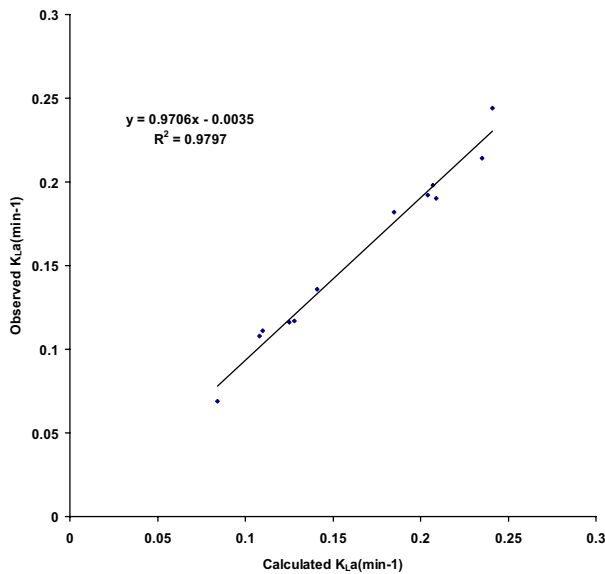
Fig. 11 Relationship between Observed Overall Transfer coefficient ( K_{L,a} ) & Calculated Overall Transfer coefficient ( K_{L,a} ).
