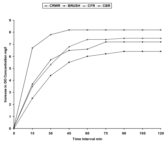
Fig. 5 Variation of Dissolve Oxygen with Time for different Aerators at speed 42 RPM and 5.5 Depth of Immersion
