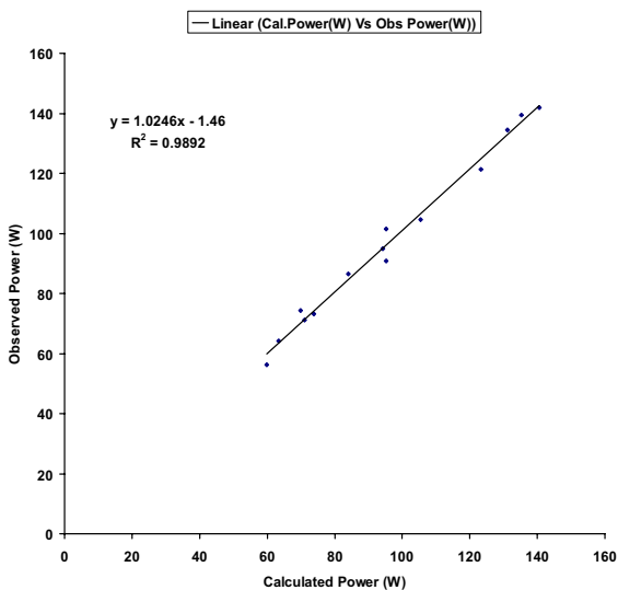
Fig. 12 Relationship between Observed power values (W) & Calculated power values (W)
