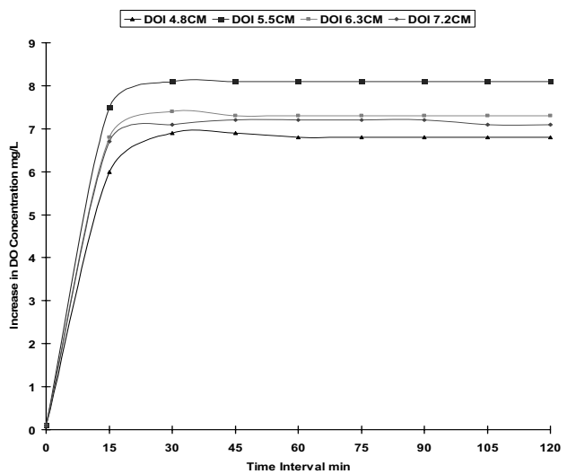
Fig. 2 Variation of Dissolve Oxygen (mg/L) with Time for Different Depth of immersion for CBR Aerator
