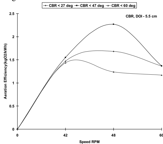
Fig. 10 Effect of Speed on Aeration efficiency for CBR aerator at depth of immersion of 5.5 cm
