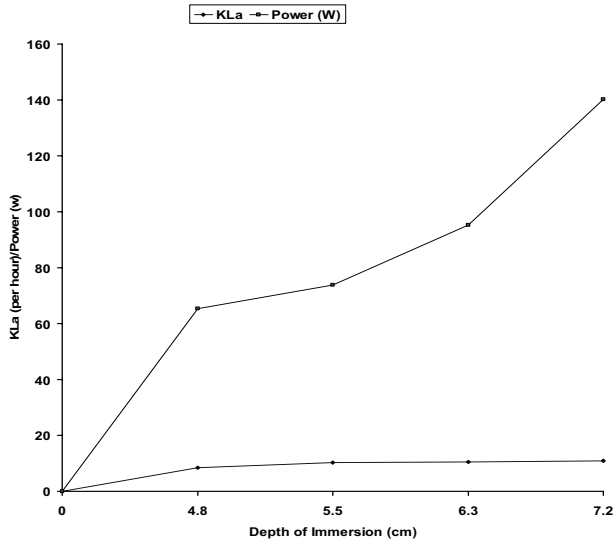
Fig. 3 Influence of Depth of Immersion on Overall Oxygen Transfer Coefficient & Power (W)
