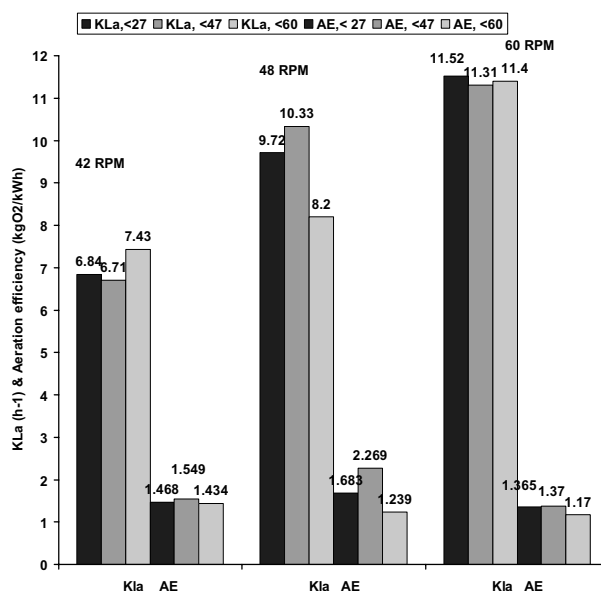
Fig. 9 Variation of K_La (h -1 ) & Aeration Efficiency (kgO 2 /kWh) For different blade angles & Speed of aerator(rpm)
