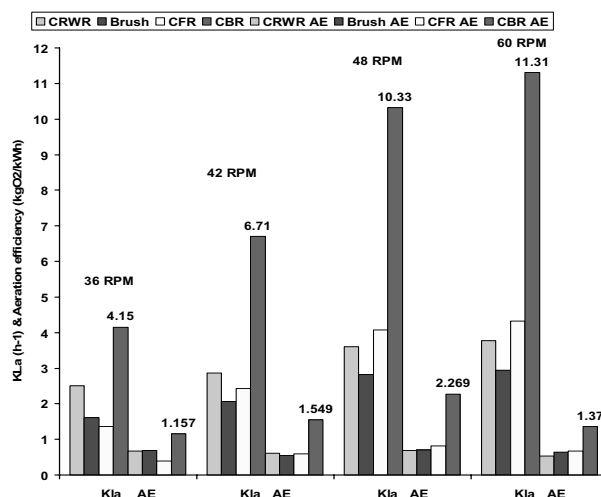
Fig. 8 Variation of K_La (h -1 ) & Aeration Efficiency(kgO 2 /kWh) with Rotor Type & Speed of aerator (RPM)
