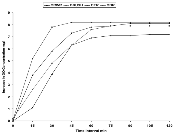
Fig. 4 Variation of Dissolve Oxygen with Time for different Aerators at speed 36 RPM and 5.5 Depth of Immersion
