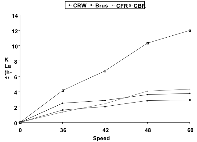
Fig. 1 Variation of over all Oxygen Transfer Coefficient K_L.a with aerator Speed for different aerators
