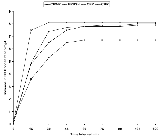
Fig. 6 Variation of Dissolve Oxygen with Time for different Aerators at speed 48 RPM and 5.5 Depth of Immersion
