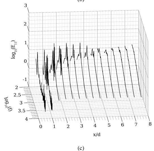
Fig. 10 One dimensional spectra at three different Reynolds numbers, (a) 4000, (b) 6000 and (c) 8000
