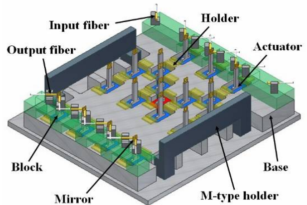
Fig. 3 The model of 8 \times 8 optical switch
