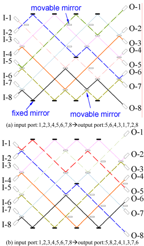
Fig. 1 The layout of the optical switch
