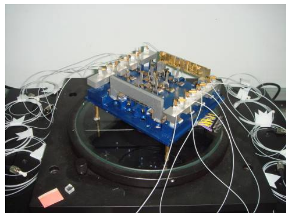
Fig. 4 Prototype of 8 \times 8 optical switch
