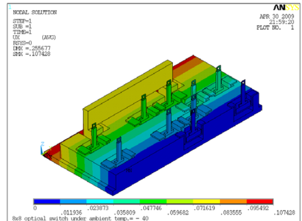
Fig. 13 Thermal deformation diagrams
