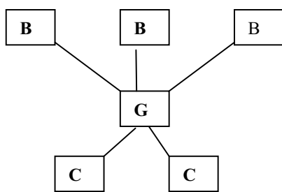
Fig. 1 B2G2C model
