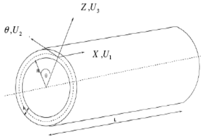
Fig. 2: Geometry of a cylindrical shell
