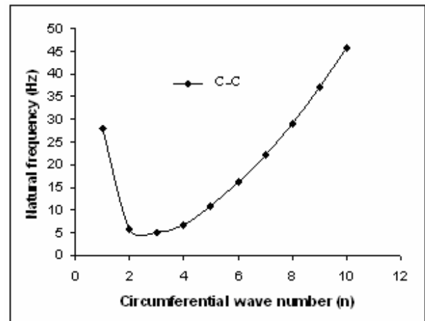
Fig. 4 Natural frequencies FG cylindrical shell associated with C-C boundary conditions. ( m=1, h/R=0.002, L/R=20 ).
