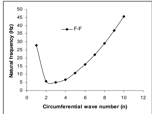
Fig. 3 Natural frequencies FG cylindrical shell associated with F-F boundary conditions. ( m=1, h/R=0.002, L/R=20 )
