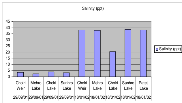
Fig. 1 Values of salinity at various lakes in the vicinity of LBOD
