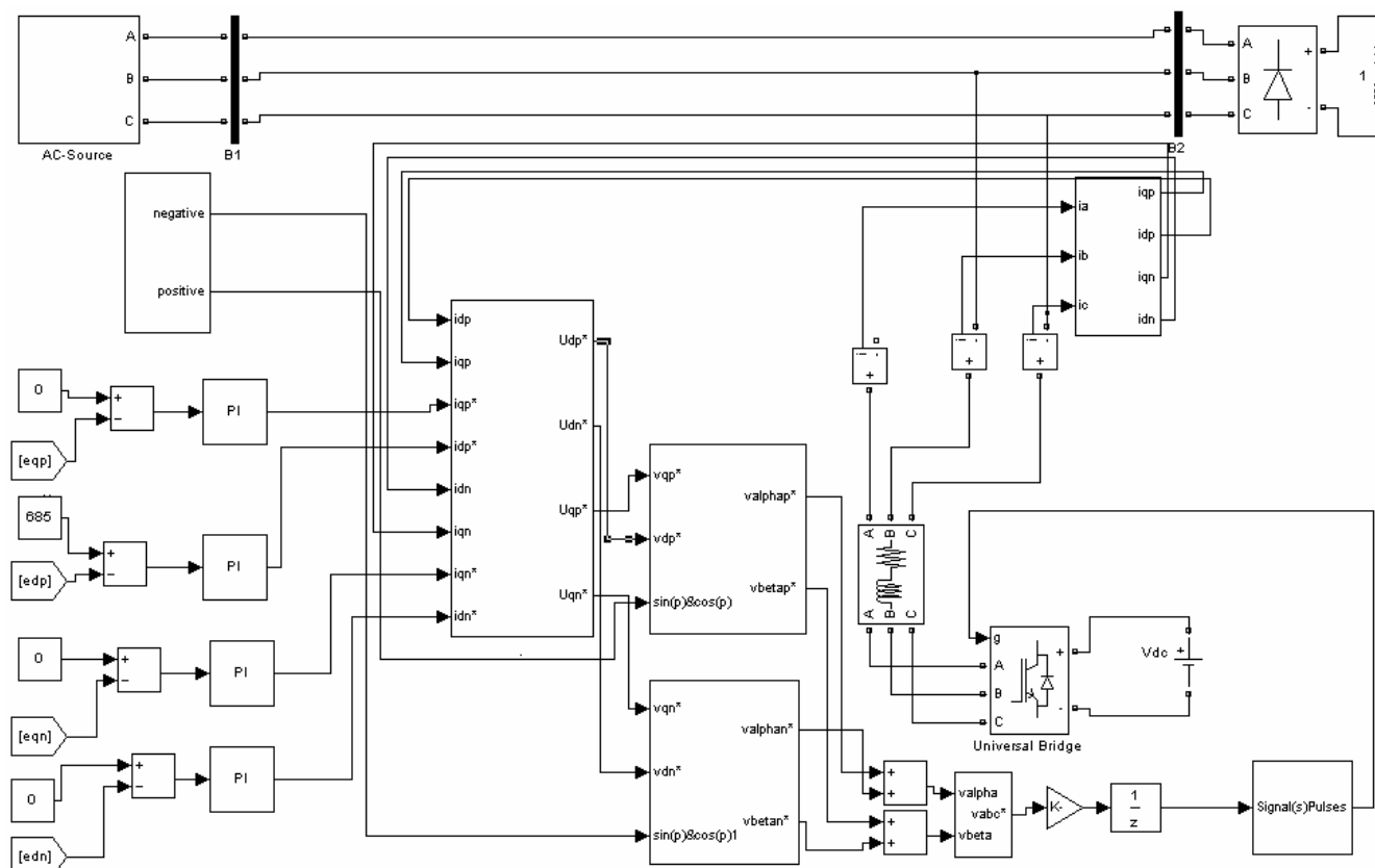
Fig. 4 Simulated DSTATCOM control system using MATLAB/SIMULINK
