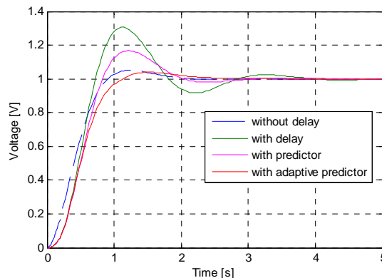
Fig. 7 Step time responses of motor voltage with PI control, predictive control and predictive control with adaptation time delay. Average value of time delay is 6*T
