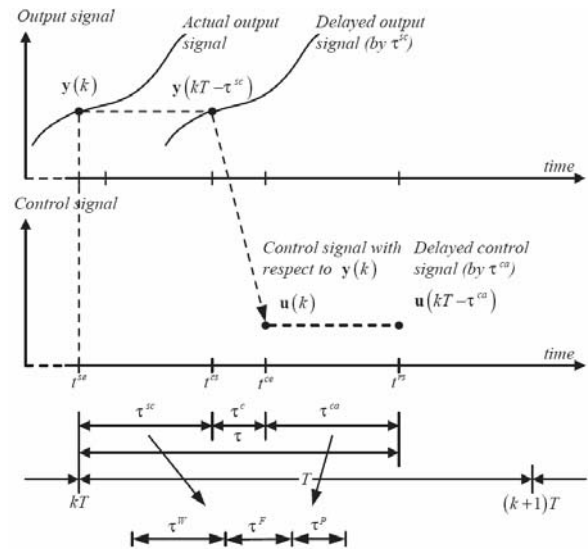
Fig. 2 Timing diagram of network delay propagations
