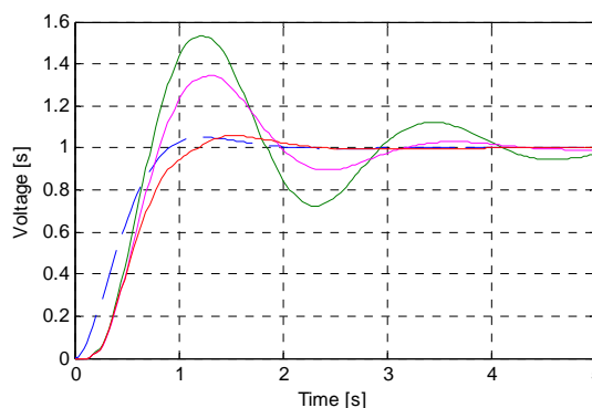
Fig. 8 Step time responses of motor voltage with PI control, predictive control and predictive control with adaptation time delay. Average value of time delay is 9*T
