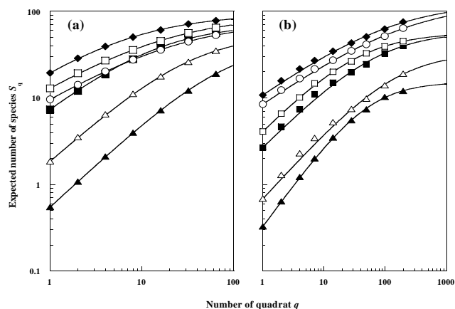
Fig. 2 Species–area curves (quadrat dimensions: 2.5 m × 2.5 m). Solid diamonds, total stand; open circles, bottom stratum; open squares, fourth stratum; solid squares, second stratum; open triangles, top stratum. The species–area curves were fit with (10), where in the Ishigaki forest (a) S_{\max} = 92 ( R^2 \cong 1.0 ) for the total stand, and S_{\max} = 88 ( R^2 \cong 1.0 ), 90 ( R^2 \cong 1.0 ), 77 ( R^2 \cong 1.0 ), 55 ( R^2 \cong 1.0 ), and 44 ( R^2 \cong 1.0 ) for the bottom through the top stratum, respectively, and in the Dinghushan forest (b) S_{\max} = 127 ( R^2 \cong 1.0 ) for the total stand, and S_{\max} = 126 ( R^2 \cong 1.0 ), 56 ( R^2 \cong 1.0 ), 57 ( R^2 \cong 1.0 ), 74 ( R^2 \cong 1.0 ), and 15 ( R^2 \cong 1.0 ) for the bottom through the top stratum, respectively
