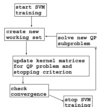
Fig. 1. Decomposition scheme for SVM training.
