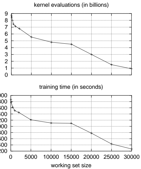
Fig. 3. Number of kernel evaluations and training time for different values of \hat{l} .
