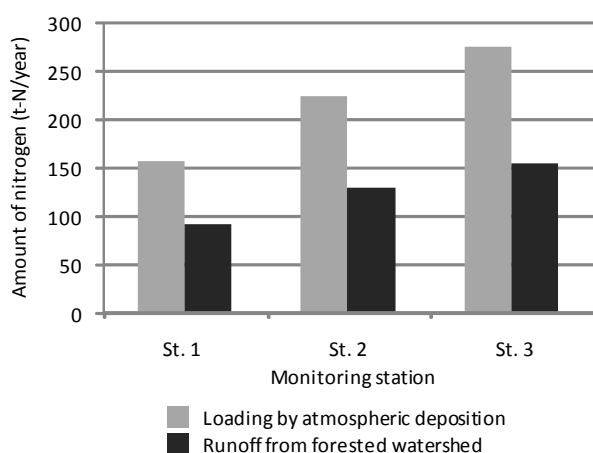
Fig. 2 Relationship between nitrogen loading and runoff estimates
