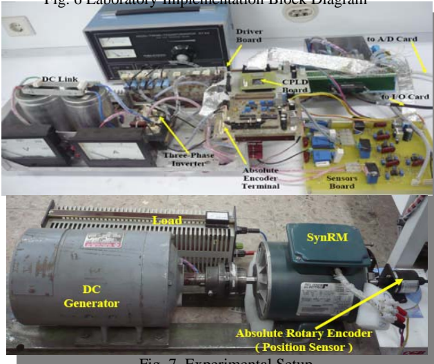
Fig. 7 Experimental Setup
