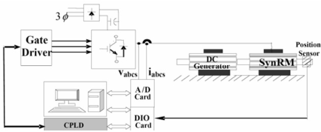
Fig. 6 Laboratory Implementation Block Diagram
