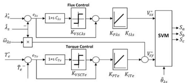
Fig. 2 Linear and Variable Structure Control (LVSC)
