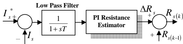
Fig. 3 PI Resistance Estimator of SynRM Drive System
