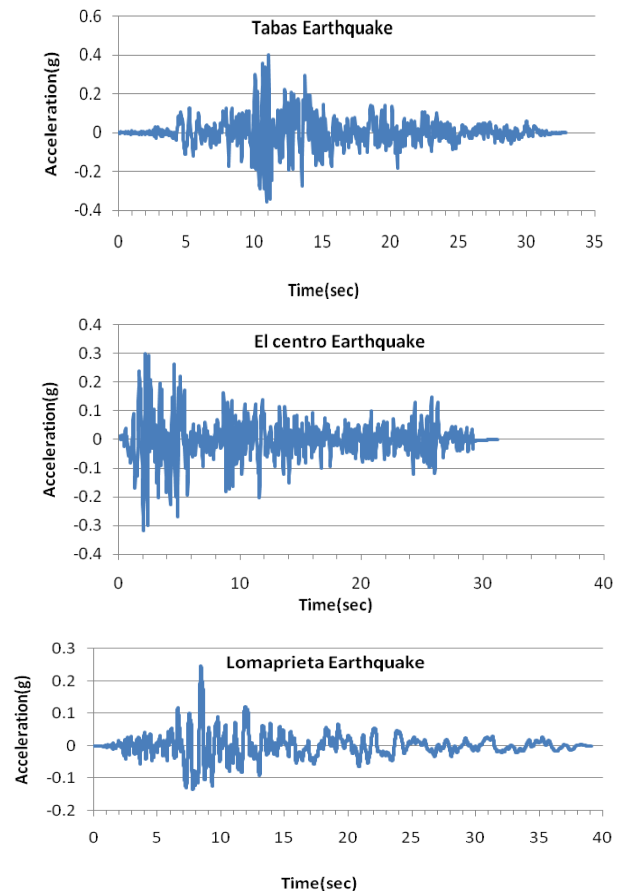
Fig. 3 Time-acceleration diagram for Tabas El centro and Lomapieta earthquake
