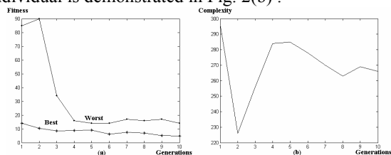
Fig. 2 (a) The achieved classification performance during the evolution process. (b) the behavior of the network complexities versus the generations.
