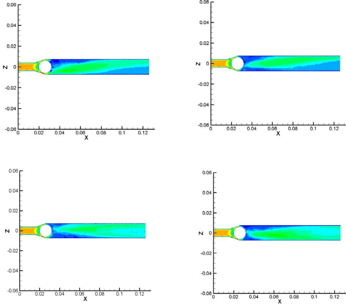
Fig. 4 Mid-section (X-Z plane) velocity field during one period of oscillation
