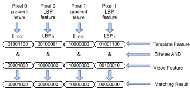
Fig. 5 Matching score bitwise operation
